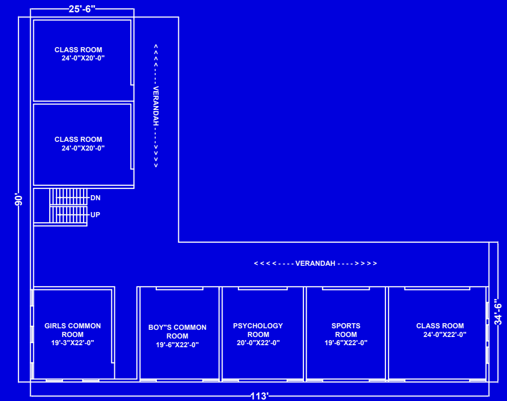
SECOND FLOOR PLAN PLAN :- 5924.25 SQ. FEET. / 550.58 SQ. MTR.
