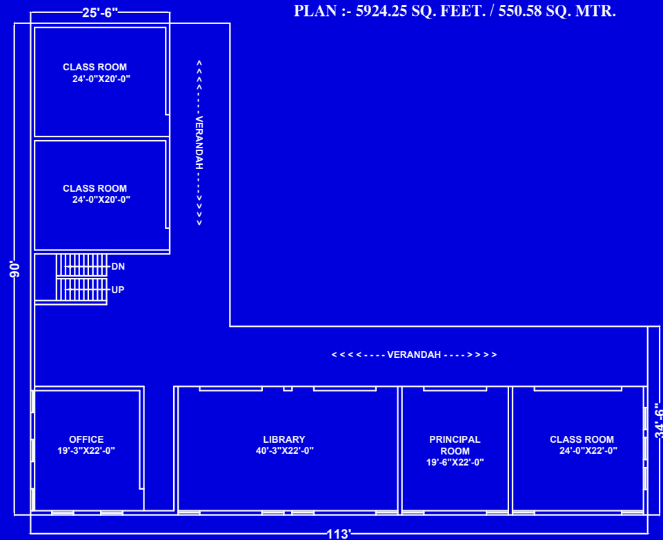
FIRST FLOOR PLAN PLAN :- 5924.25 SQ. FEET. / 550.58 SQ. MTR.
