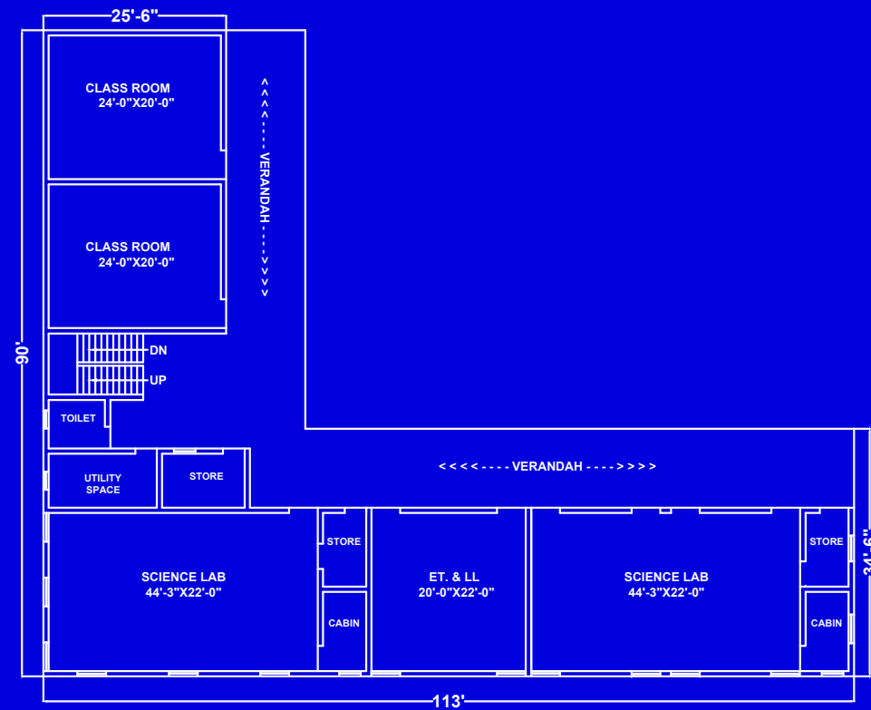
GROUND FLOOR PLAN PLAN :- 5924.25 SQ. FEET. / 550.58 SQ. MTR.
